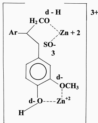
ZINC LIGNOSULFONATE MOLECULE
