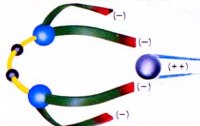
Figure 3 — The completed basic structure of EDTA.
